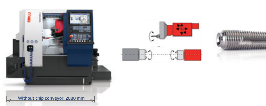
MAXXTURN 45
